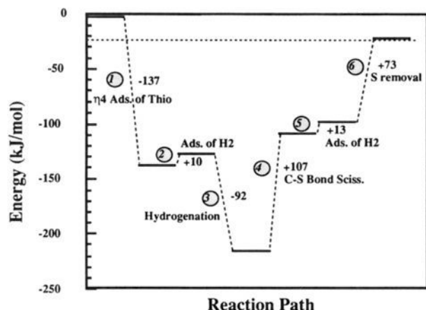
Figure 12. Proposed catalytic HDS cycle 3 for the η 4 -adsorbed thiophene and η 3 -2,5-dihydrothiophene intermediates on Ni 3 S 2 : (A) optimized structures for each step of the catalytic reaction path and (B) corresponding energies for each step.
