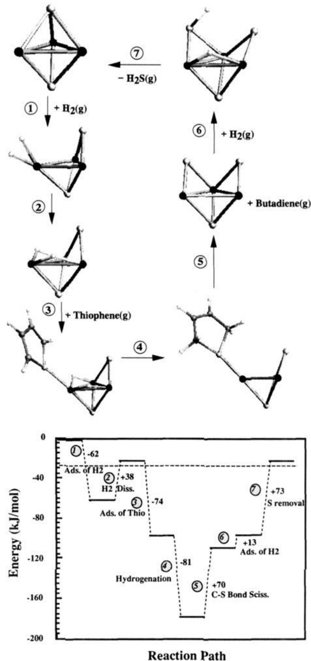
Figure 11. Proposed catalytic HDS cycle 2 for the \eta^1 -adsorbed thiophene and 2,5-dihydrothiophene intermediates on \text{Ni}_3\text{S}_2 ( \text{H}_2 adsorption initiated): (A) optimized structures for each step of the catalytic reaction path and (B) corresponding energies for each step.
