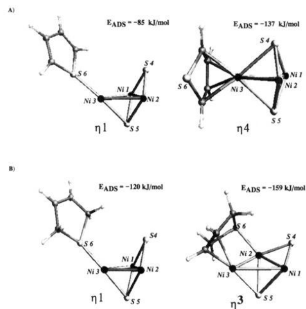
Figure 8. Adsorption of thiophene and 2,5-dihydrothiophene on \text{Ni}_3\text{S}_2 : (A) adsorption of thiophene in \eta^1 and \eta^4 configurations and (B) adsorption of 2,5-dihydrothiophene in \eta^1 and \eta^3 configurations.
