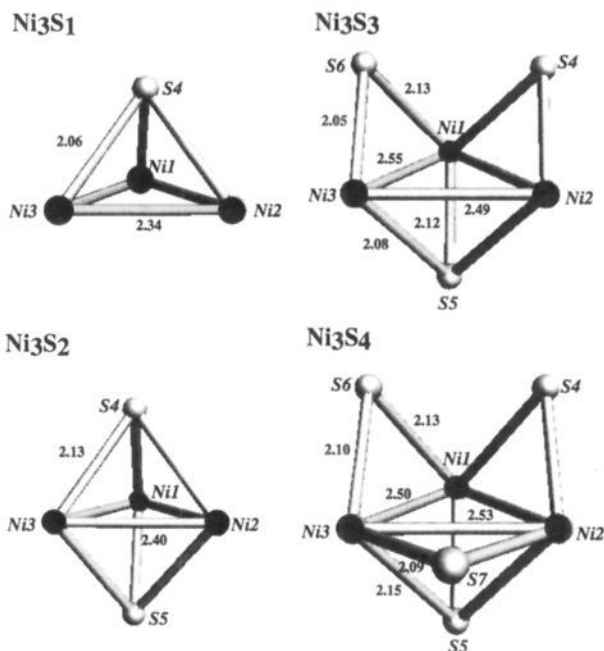
Figure 1. Optimized structures of Ni 3 S y .
