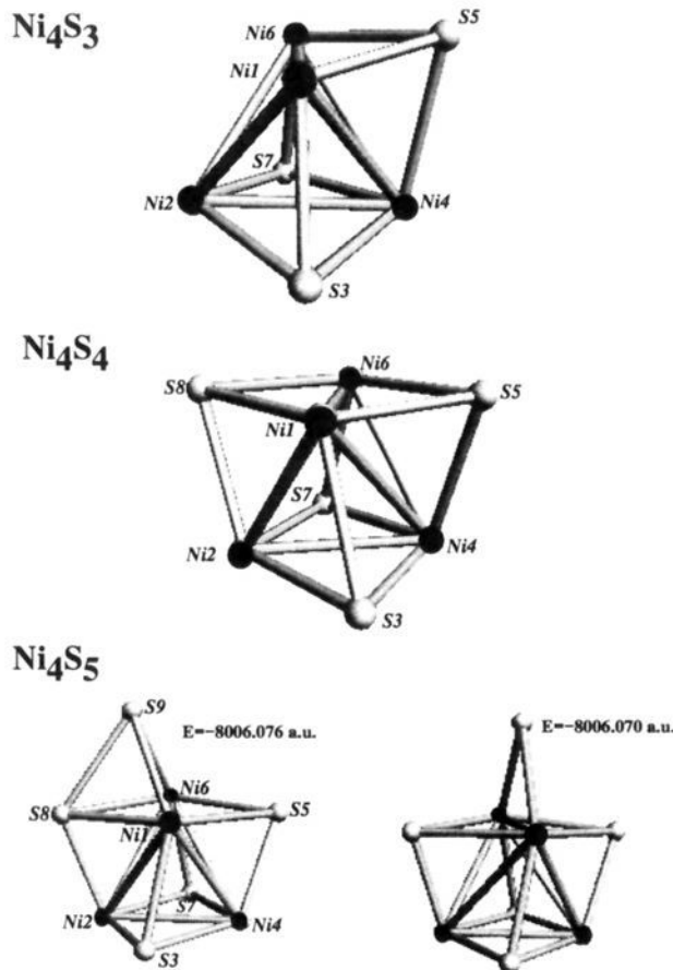
Figure 2. Optimized structures of Ni_4S_x .
