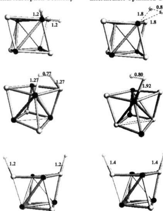
Figure 9. Attempted adsorption of H 2 on Ni 4 S 4 .
