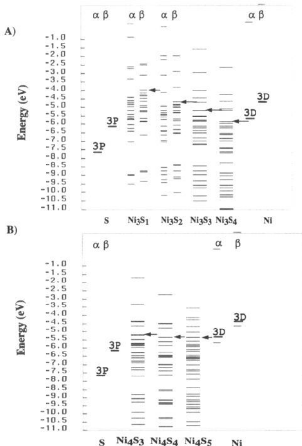
Figure 3. Orbital energy spectra for the eigenvalues closest to the highest and lowest MOs for the Ni 3 S y and Ni 4 S y clusters.
