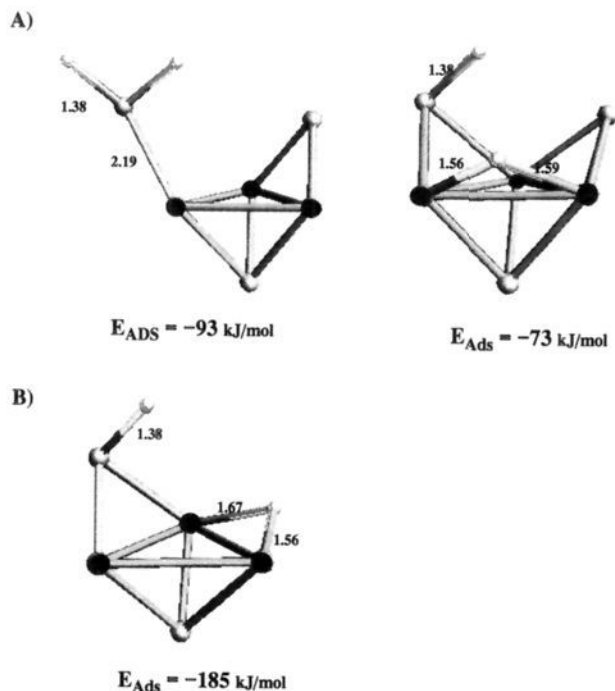
Figure 7. Adsorption of hydrogen sulfide on \text{Ni}_3\text{S}_y clusters: (A) molecular and dissociative adsorption of \text{H}_2\text{S} over \text{Ni}_3\text{S}_2 and (B) dissociative adsorption of \text{H}_2\text{S} over \text{Ni}_3\text{S}_3 .
