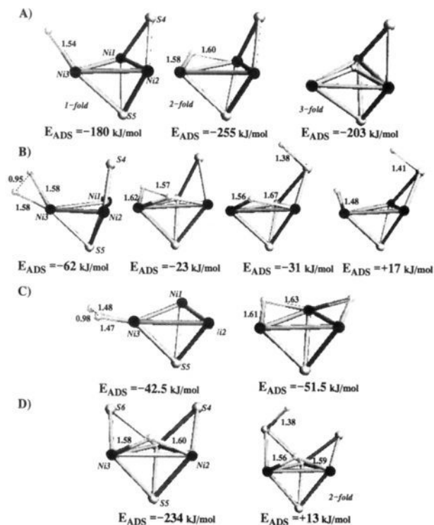
Figure 5. Adsorption of (A) atomic hydrogen on \text{Ni}_3\text{S}_2 , (B) \text{H}_2 on \text{Ni}_3\text{S}_2 , (C) \text{H}_2 on \text{Ni}_3\text{S}_1 , and (D) atomic hydrogen on \text{Ni}_3\text{S}_3 .
