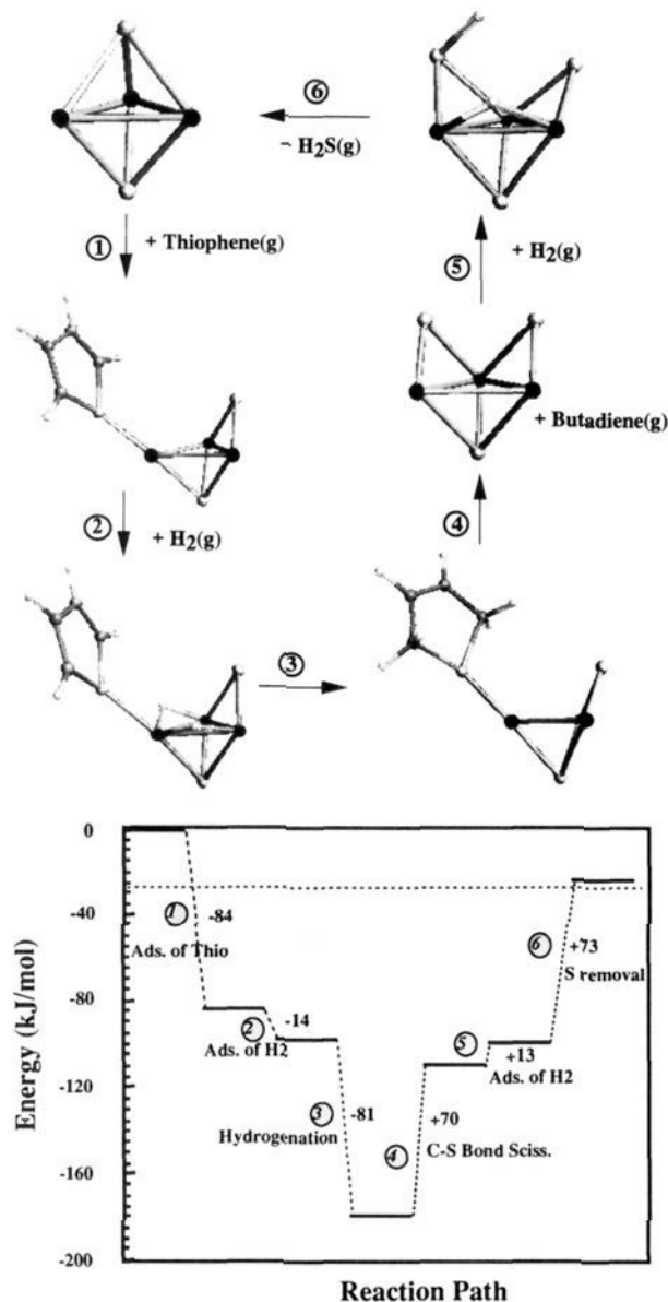
Figure 10. Proposed catalytic HDS cycle 1 for the \eta^1 -adsorbed thiophene and 2,5-dihydrothiophene intermediates on \text{Ni}_3\text{S}_2 (thiophene adsorption initiated): (A) optimized structures for each step of the catalytic reaction path and (B) corresponding energies for each step.
