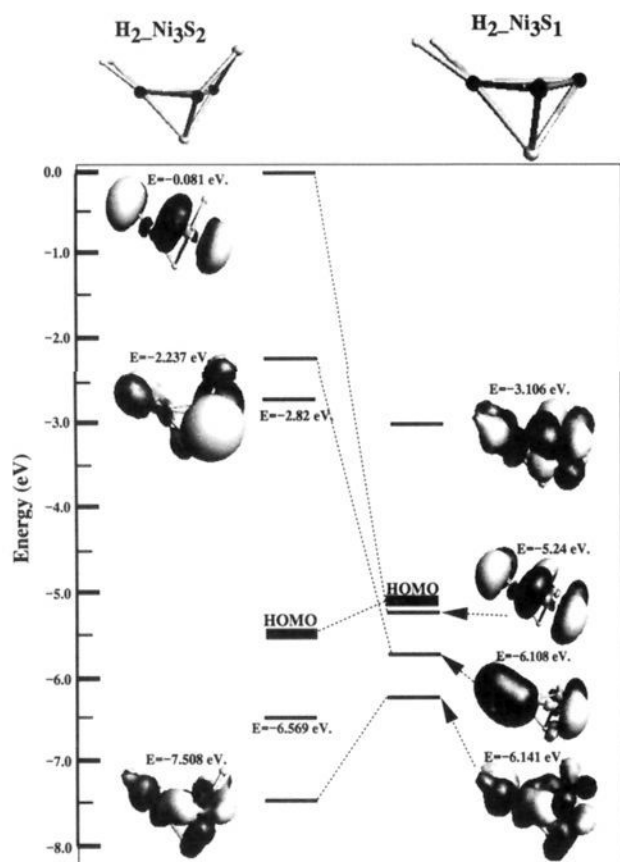
Figure 6. Frontier orbitals with substantial \text{H}_2 antibonding character in the adsorption of hydrogen on \text{Ni}_3\text{S}_2 and \text{Ni}_3\text{S}_1 . The underlying geometry for both \text{H}_2 - \text{Ni}_3\text{S}_2 and \text{H}_2 - \text{Ni}_3\text{S}_1 clusters are depicted at the top of the page.
