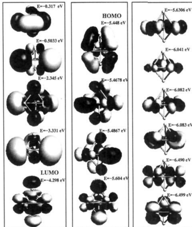
Figure 4. Molecular orbitals closest to the highest and lowest occupied orbital for the Ni 3 S 2 cluster.
